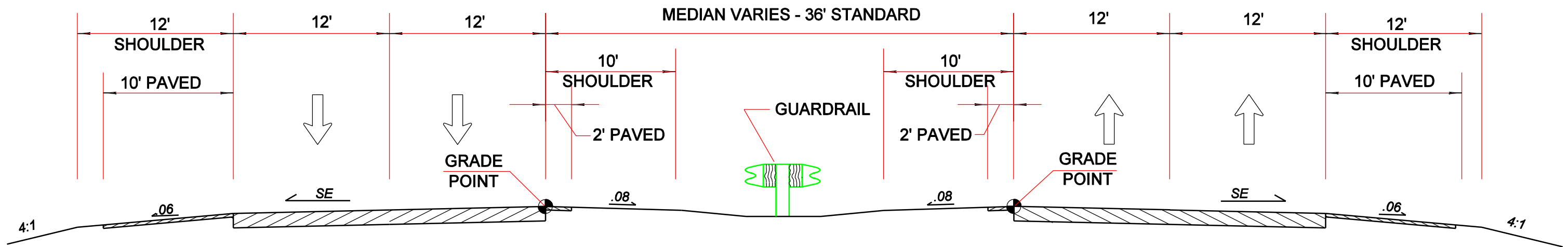
TYPICAL SECTION SOUTH OF PATTERSON AVENUE TO NORTHERN CITY LIMIT
