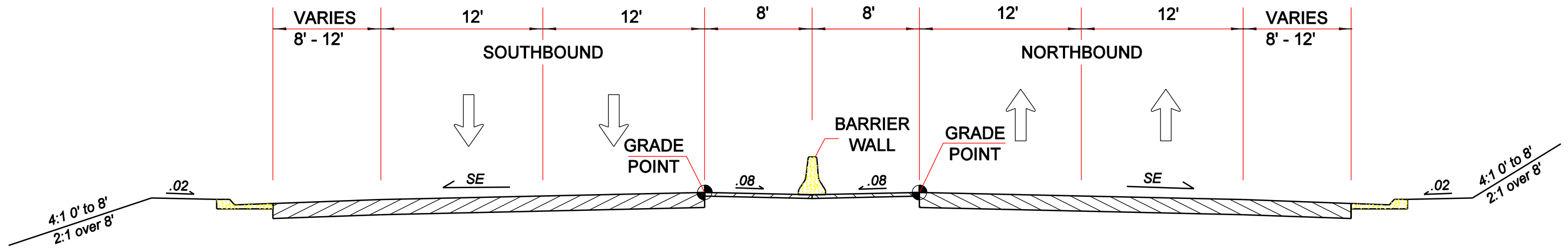
TYPICAL SECTION I-40 TO SOUTH OF PATTERSON AVENUE
